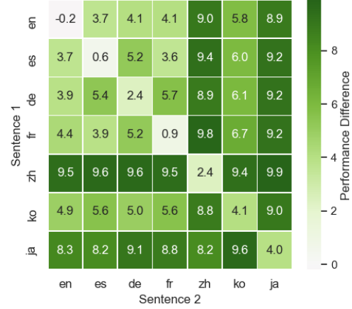
(b) mBERT-RS-DA
