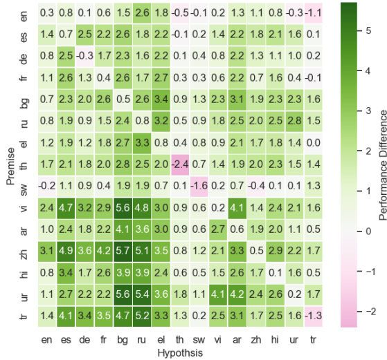
(a) mBERT-RS-RP
